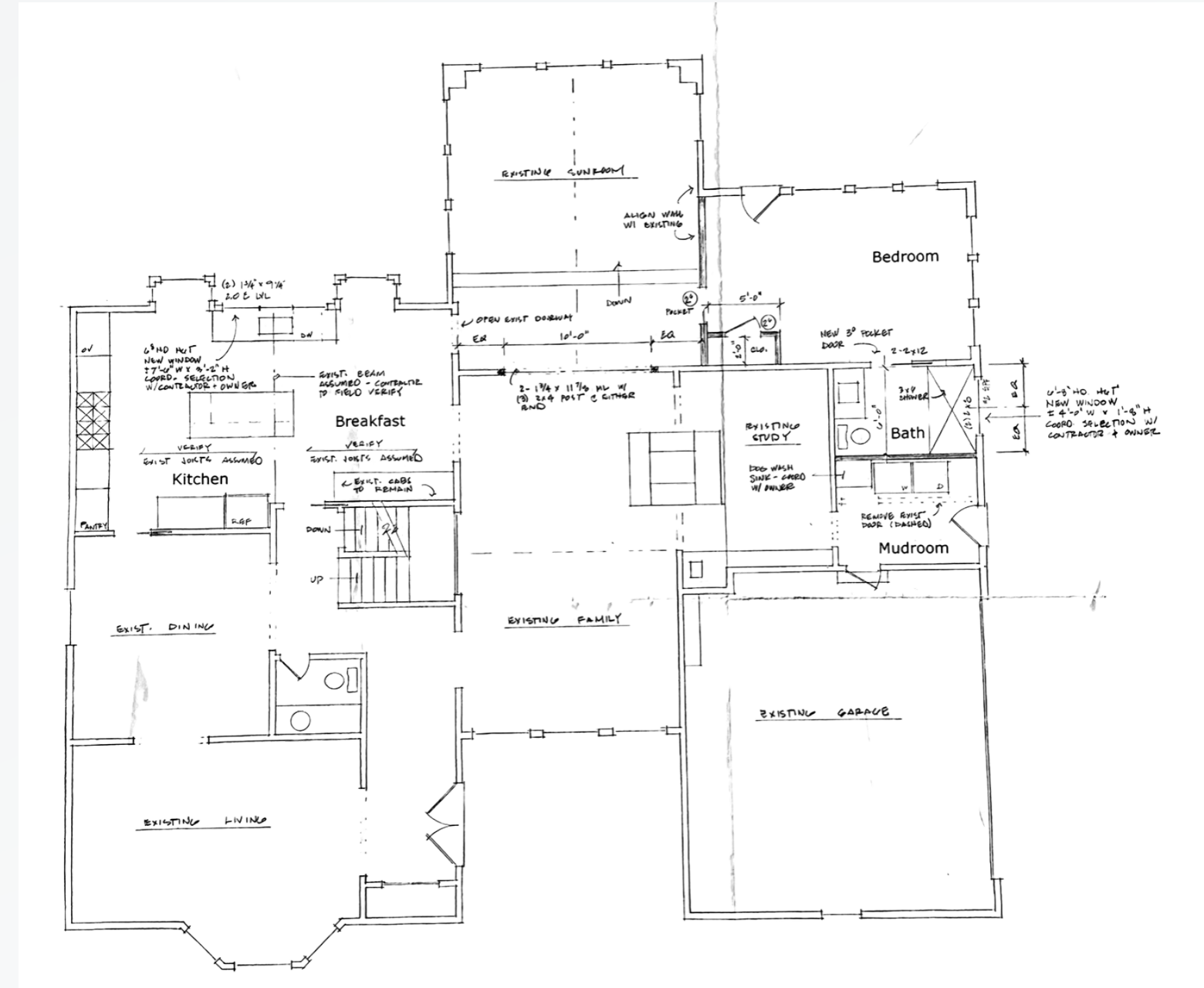
HOME LAYOUT: AFTER REMODEL
