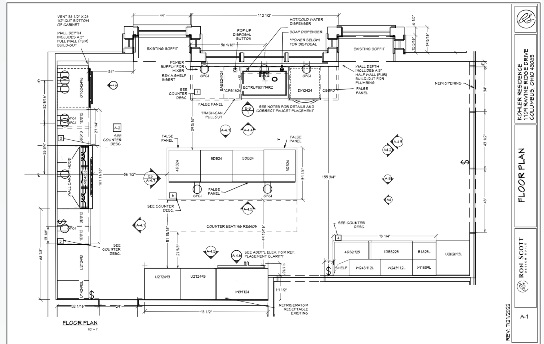
KITCHEN DESIGN AFTER REMODEL
